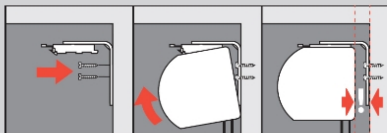
Wandmontage
